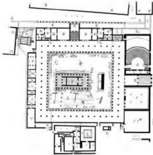
Fig. 7 — Ground plan of the sanctuary of Asklepios.
